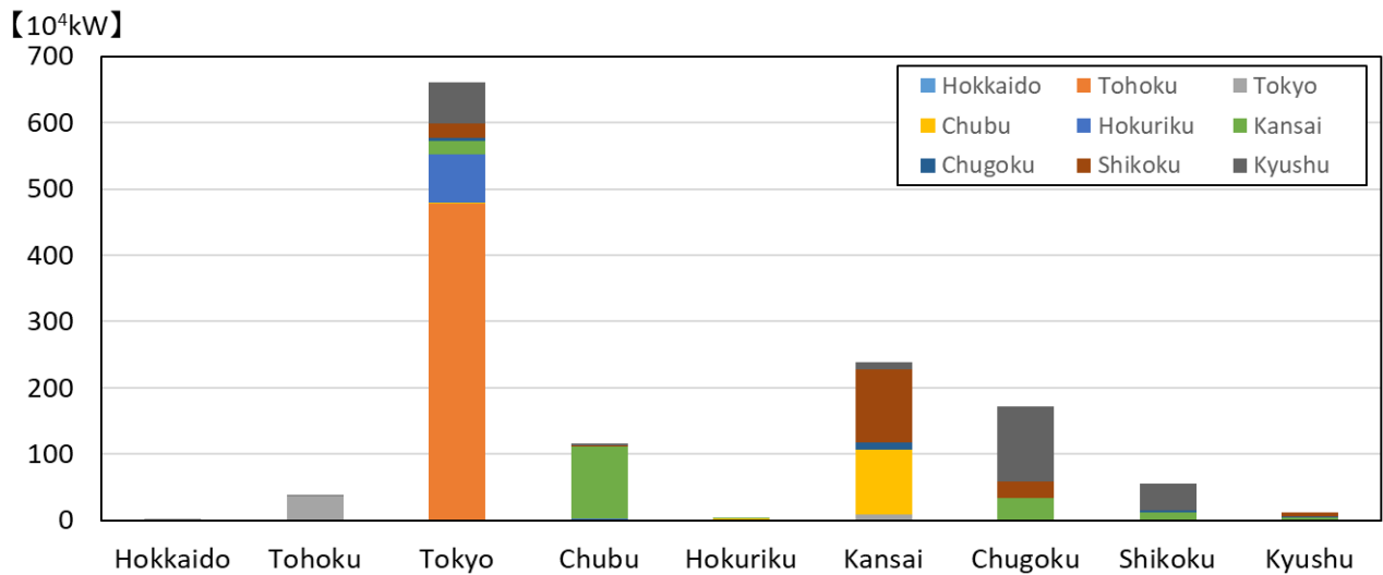
Figure 5-1 Scheduled Procurement of Supply Capacity from External Regional Service Areas
